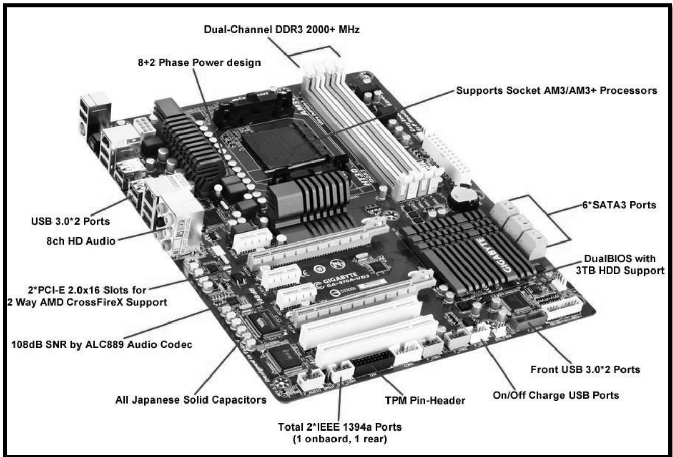
Motherboard
