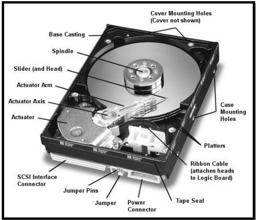
Hard Disk
